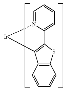
Ir(btp) 3
