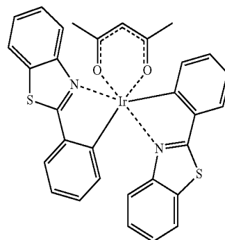
(bt) 2 Ir(III)(acac)
