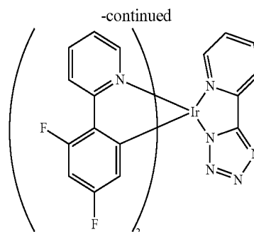
Iridium (III) bis(4,6-difluorophenylpyridinato)-5-(pyridine-2-yl)-1H-tetrazolate (FlrN4)
