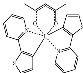
(thp) 2 Ir(III)(acac)
