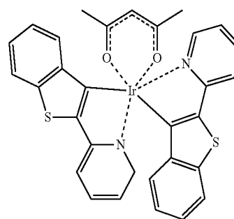
Ir(btp) 2 (acac)
