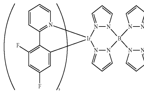
bis[2-(4,6-difluorophenyl)pyridinato-N,C2']iridium(III)tetra(1-pyrazolyl)borate (Fir6)
