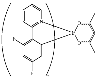
bis(2-[4,6-difluorophenyl]pyridinato-N,C2')iridium(acetylacetonate) [Flr(acac)]
